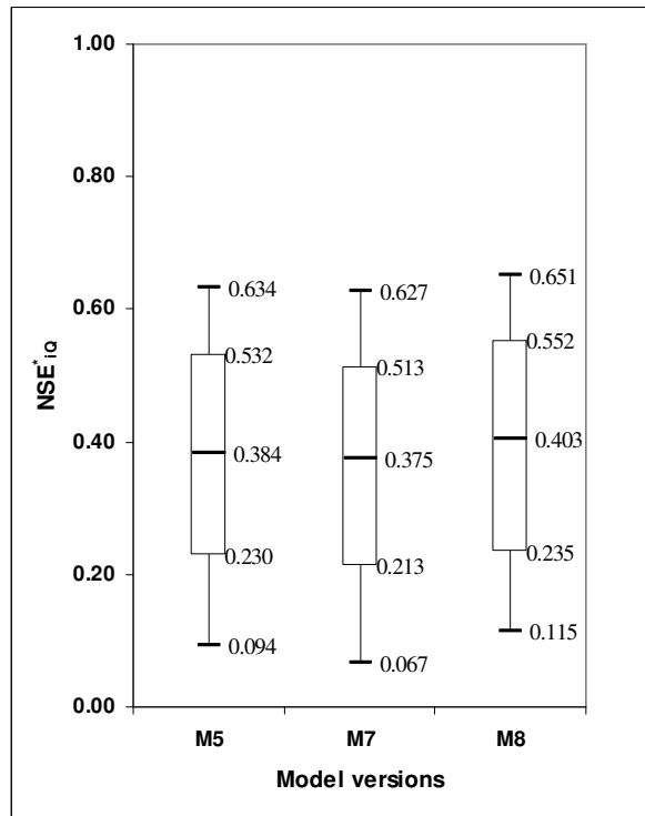
Figure 4.5: Box plots of NSE*IQ values obtained in validation by model versions having different formulations of the additional routing store (boxes represent the 0.25 and 0.75 percentiles, with the median value inside, and the whiskers represent the 0.10 and 0.90
