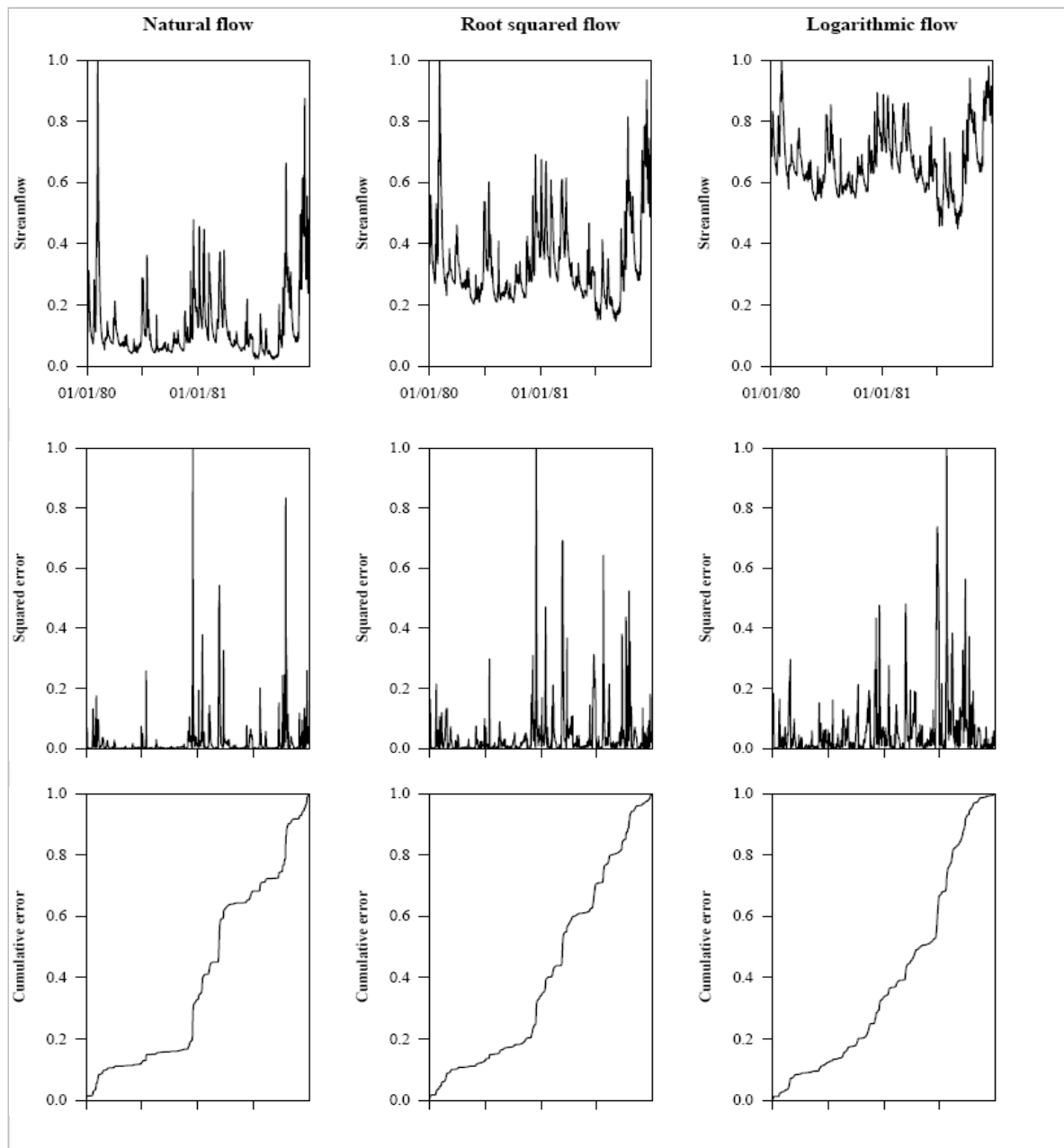
Figure 3.1: Illustration of changes in the series of flows, model errors and cumulated squared errors using root square and logarithm transformations for the Moselle River at Custines (Hydro code: A7010610; catchment area: 6830 km 2 ; period: 01/01/1980–31/12/1981).
