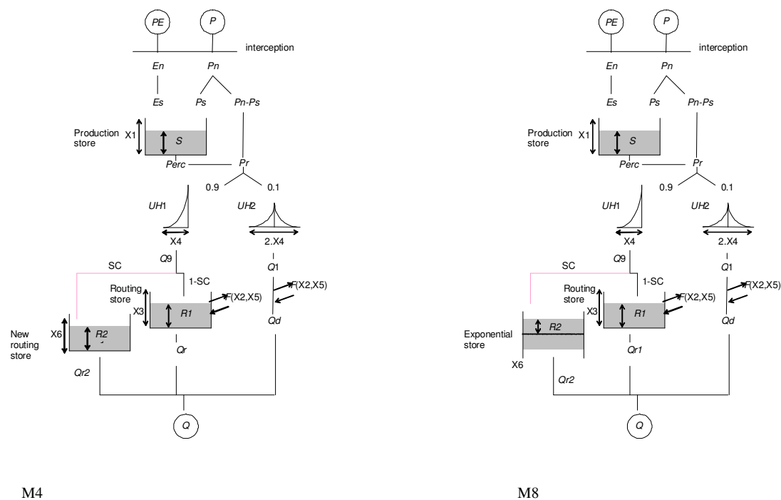
Figure 4.2: Layout of two versions of the GR5J model with different additional stores
