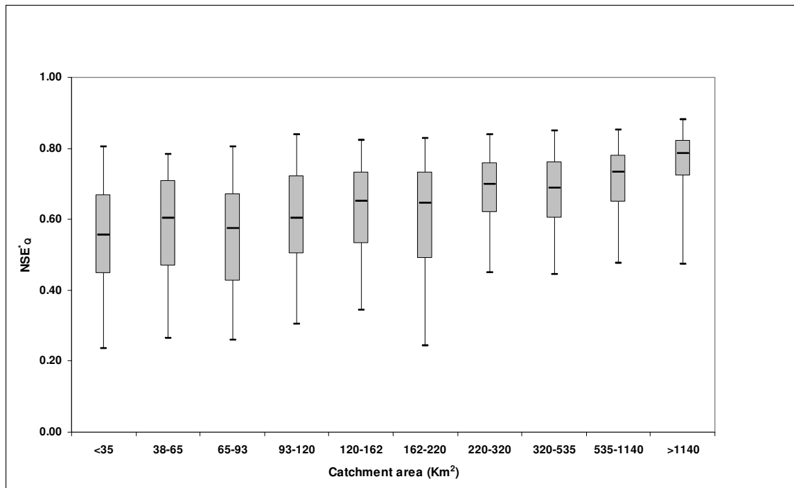
Figure 3.3: Box plots of performance ( NSE_o^* in validation) of the GR4J model on the 940 catchments as a function of catchment size (boxplots show the 0.05, 0.25, 0.5, 0.75 and 0.95 percentiles from bottom to top; each box plot contains one tenth of catchments)
