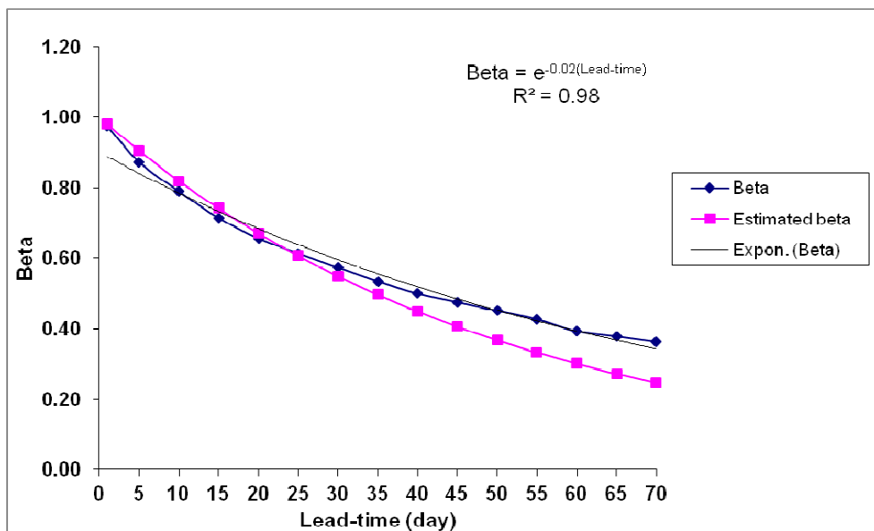
Figure 5.10: Dependency of beta value with forecast lead-time
