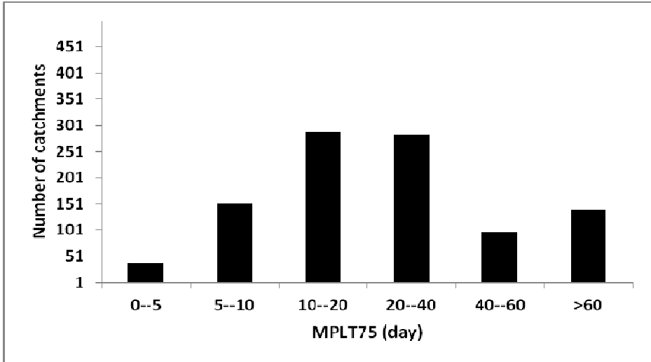
Figure 5.17: Distribution of the maximum possible lead time for the catchments on the data set
