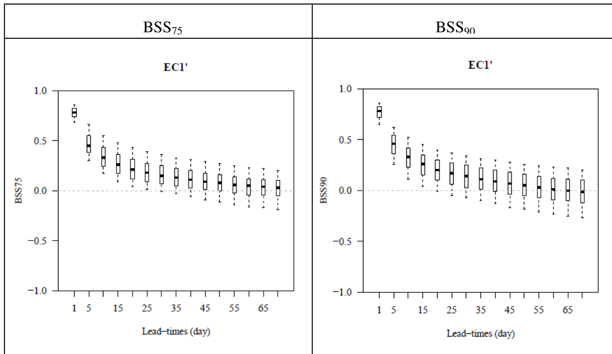
Figure 5.11: Forecast skill score with lead-time using model updating, ECI'
