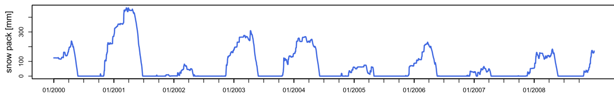
Figure 16: Snow water equivalent values on the validation period for the simulation of TUWmodel on the catchment “L’Ubaye à Lauzet-Ubaye”.
