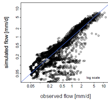
(f) TUWmodel.
